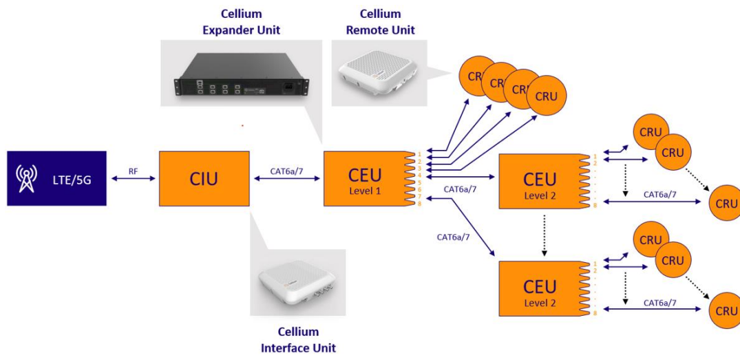
Figure: EdgeAir “C” Family Solution
